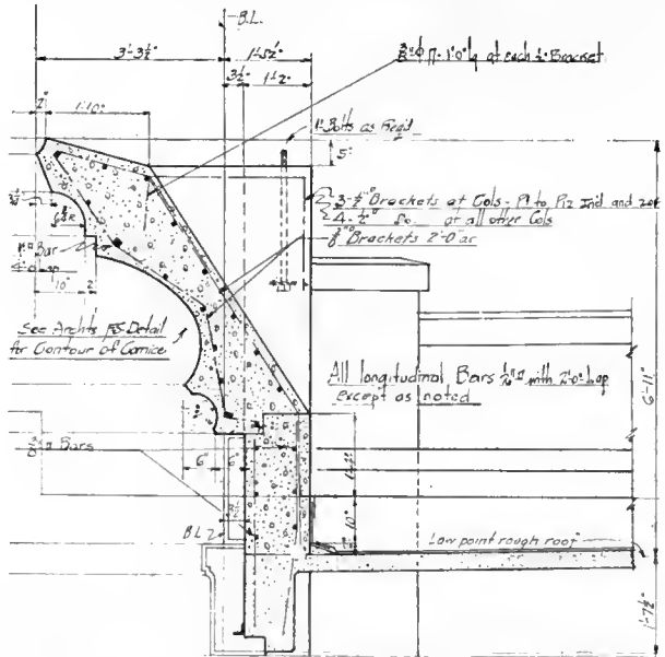
SECTION THROUGH REINFORCED CONCRETE CORNICE
